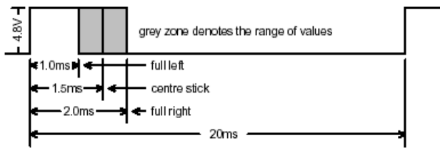
Figure 10: servo control frame waveform.
