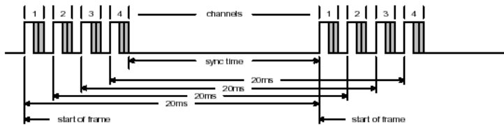
Figure 11: an example of multi-channel (4) frame.
